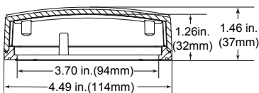
Flush Mount Side View
